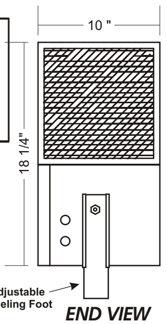
Filter/Blower Housing
